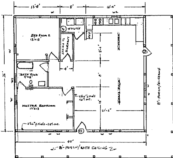
FLOOR PLAN / WITH STAIRS TO BASEMENT
