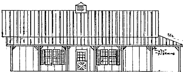
FRONT ELEVATION
